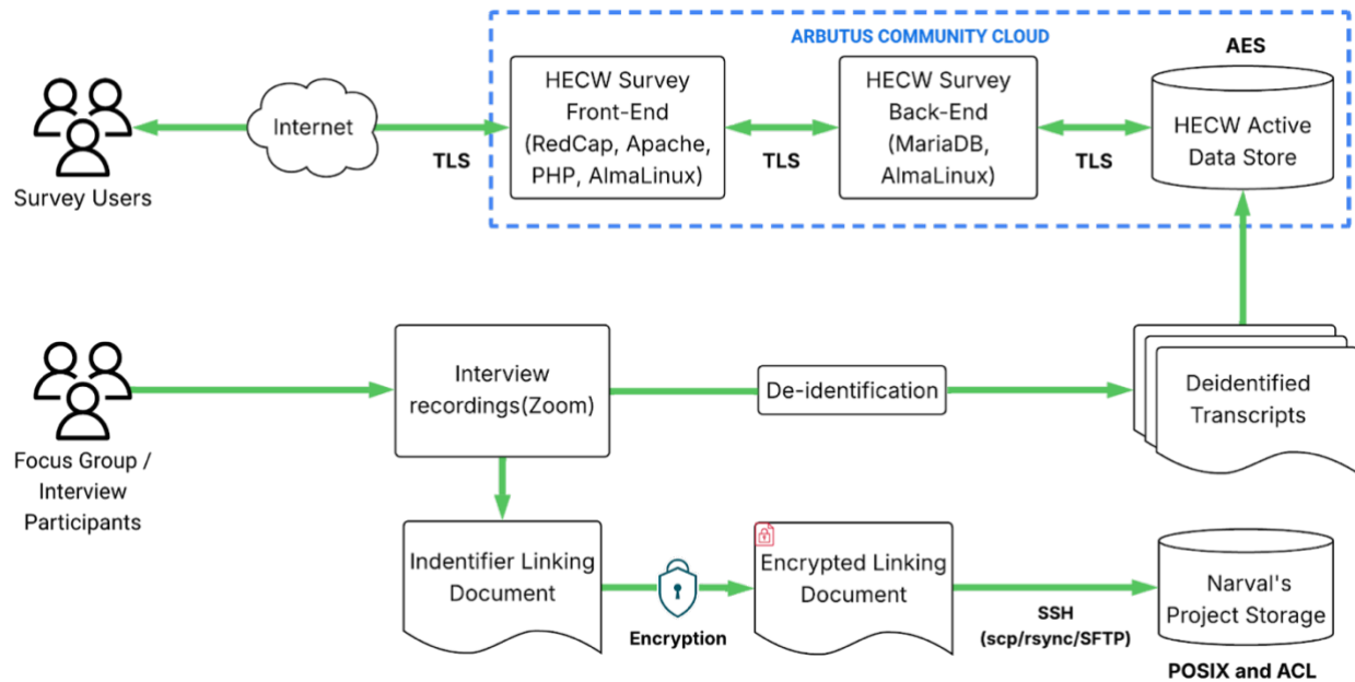
Fig. Project Architecture (Surveys + Focus Groups/Interviews - Identifiers retained)
