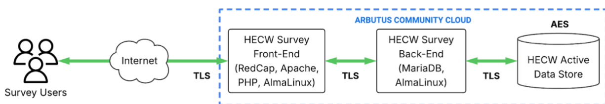
Fig. Project Architecture (Surveys Only using Redcap)
