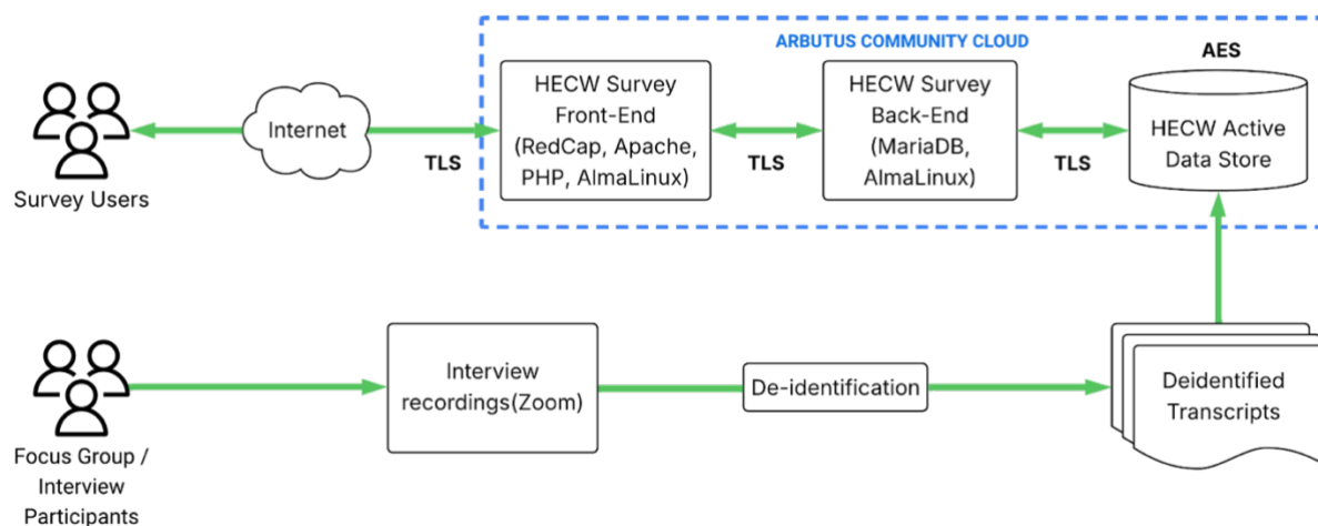
Fig. Project Architecture (Surveys + Focus Groups/Interviews - Identifiers Destroyed)
